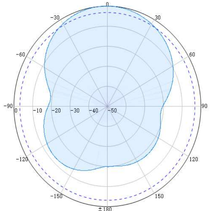
Vertical (866MHz)
